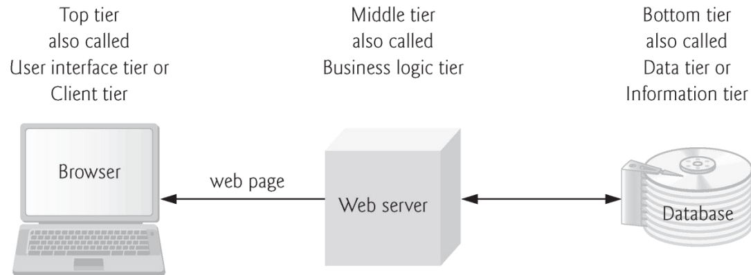
Fig. 17.3 | Three-tier architecture.
